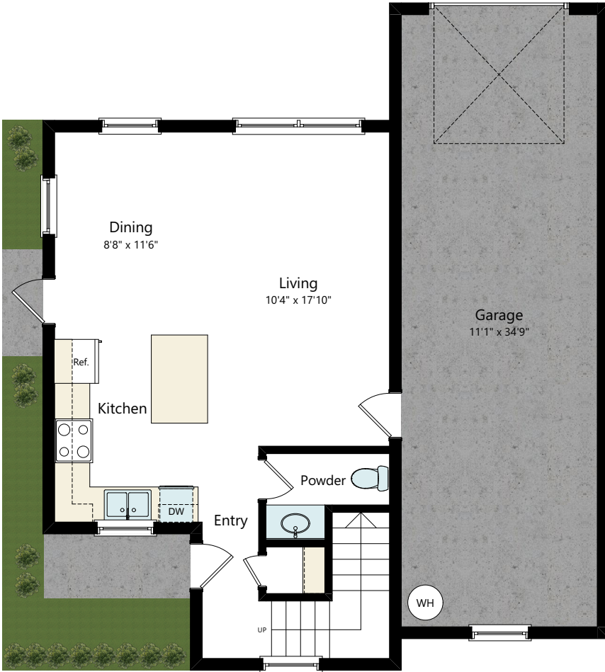
LEVEL 1
